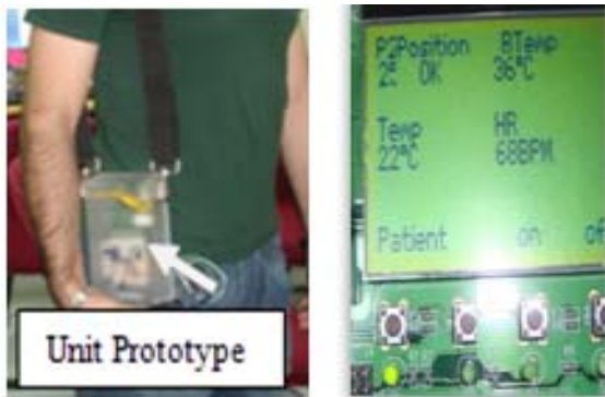
Figure 3. (a) P-Node unit and (b) M-Node screen.
