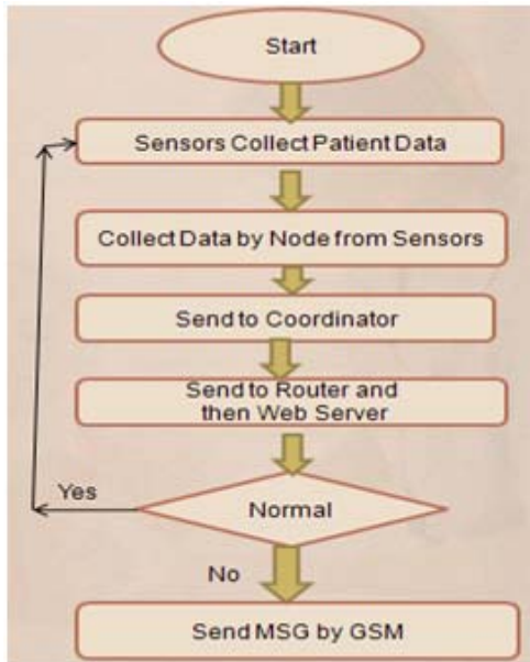
Figure 5. Data Flow Flowchart
