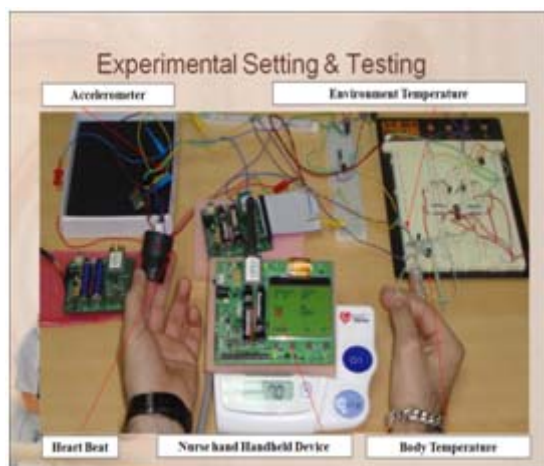
Figure 6. System Experimental Setup.
