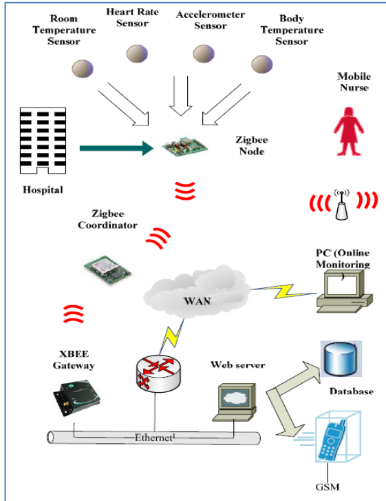
Figure 2. System Hardware Architecture
